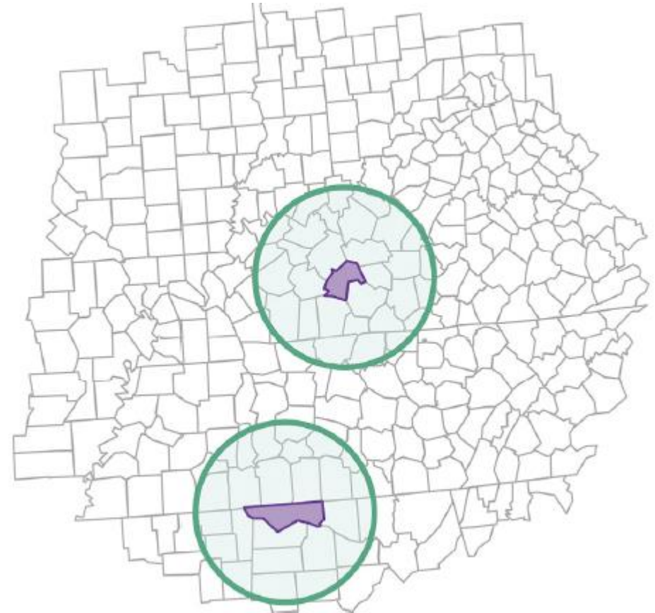
Fixed distance
