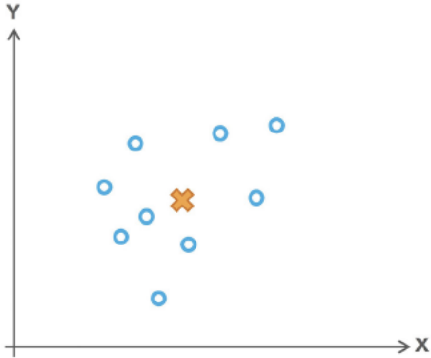
mean center
